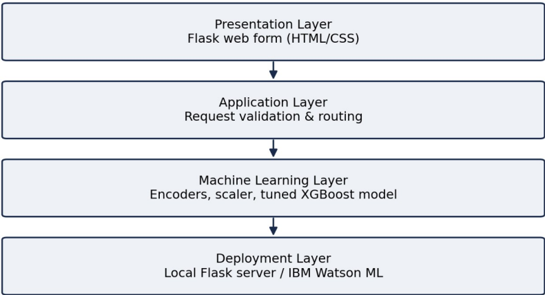
Figure 2: System architecture
